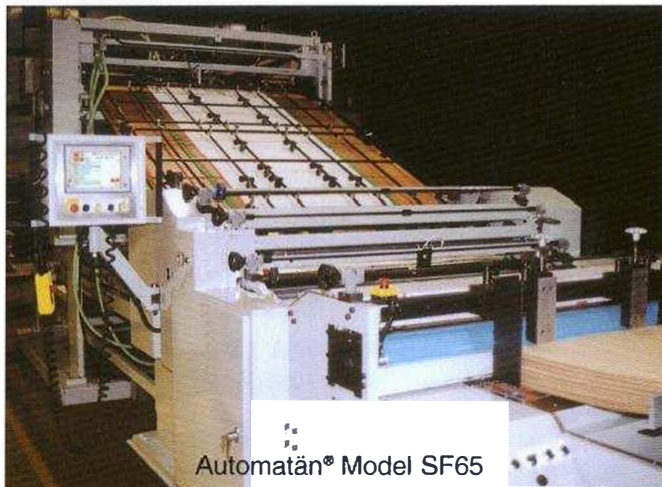
The SF65 features re-registration of the label for precision sheet-to-sheet and full mount laminating.
